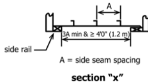
section "x" FIG. 1 General Arrangement of Air Leakage Apparatus
